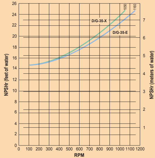
Net Positive Suction Head (NPSHr)
