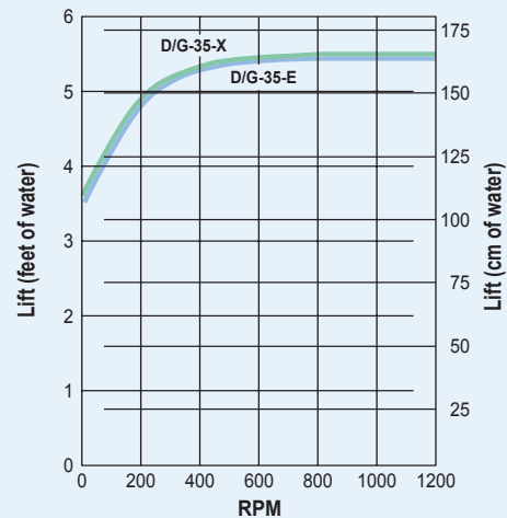
Dry Lift
